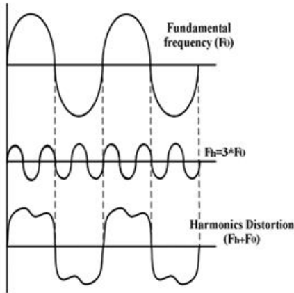
Figure 6: Harmonic distortion
